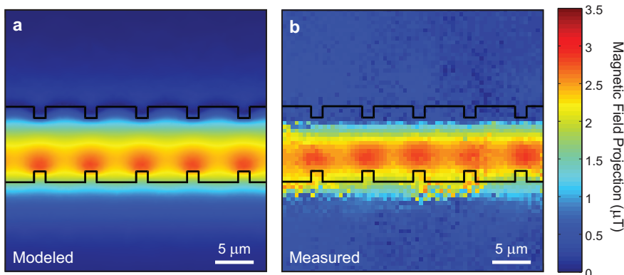
Figure 4.2: (a) Modeled and (b) measured map of the magnetic field projection along the NV axis produced by running an AC current of frequency 109.5 kHz and amplitude 50 \mu\text{A} through the notched wire pattern at a stand-off distance \approx 1 \mu\text{m} .
