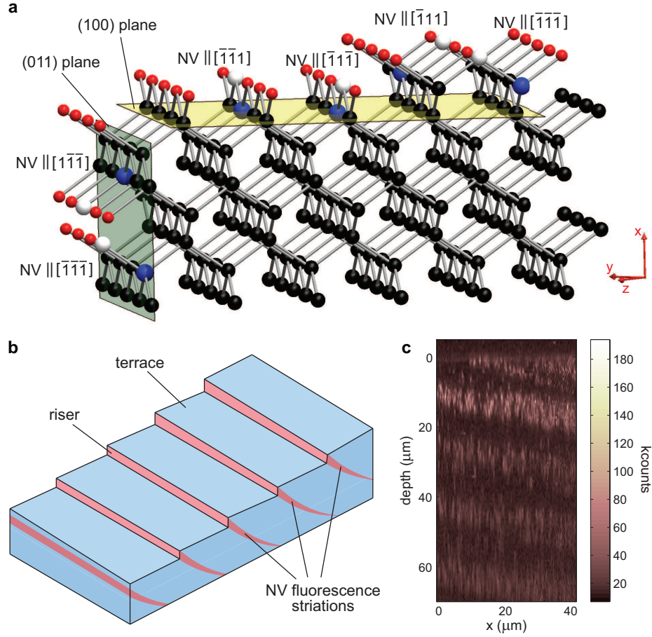
Figure 5.3: (a) Atomic-level model of NV incorporation in (100) step-flow growth, indicating mechanism for preferential NV occupation of only two orientations. (b) Diagram of {100} step-flow growth surface and fluorescence striations. (c) Confocal cross-section of a sample which exhibits fluorescence striations characteristic of {100} step-flow growth.
