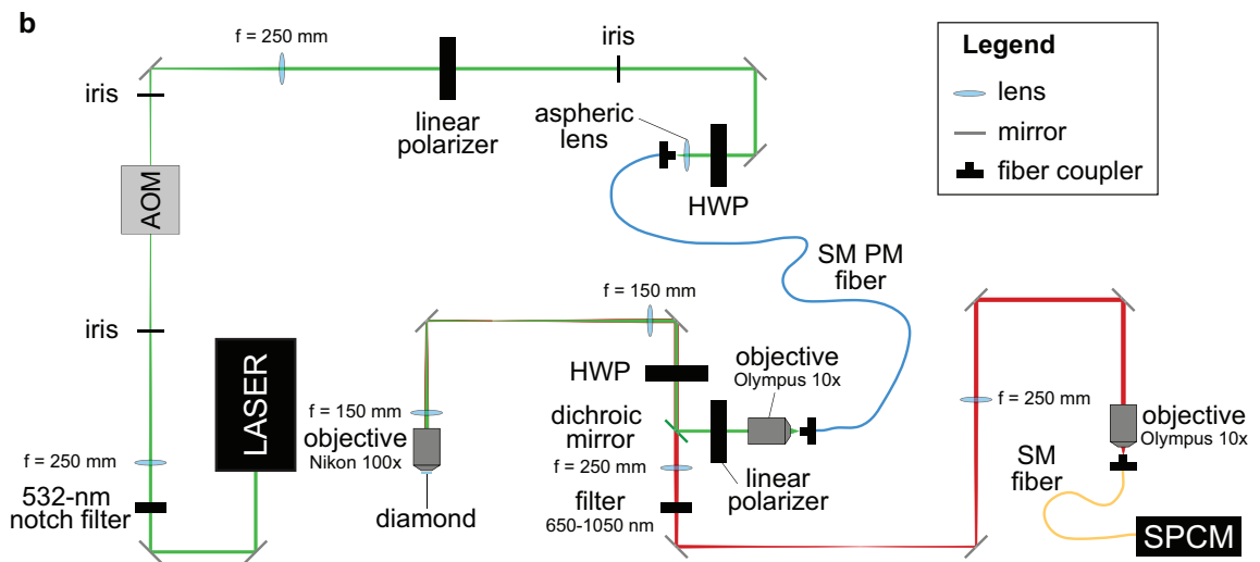
Figure B.2: NV scanning confocal microscope (a) photograph and (b) schematic.
