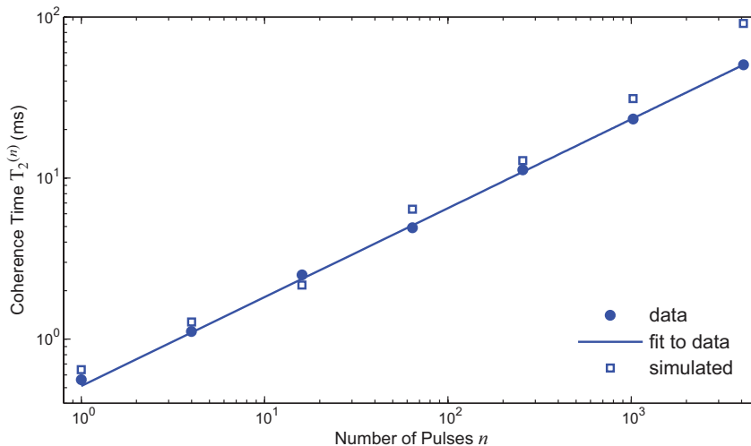
Figure 7.4: Scaling of T_2^{(n)} with the number n of CPMG pulses: derived from NV spin coherence decay data C_n(t) (dots); fit of dots to a power law T_2^{(n)} = (0.54 \pm 0.02 \text{ ms})n^{(0.54 \pm 0.01)} (solid line); and synthesized from the average-fit Lorentzian spin bath spectrum with \Delta = 12 \text{ kHz} , \tau_c = 52 \mu\text{s} (open squares), which yields a consistent fit T_2^{(n)} = (0.54 \pm 0.08 \text{ ms})n^{(0.59 \pm 0.03)} .
