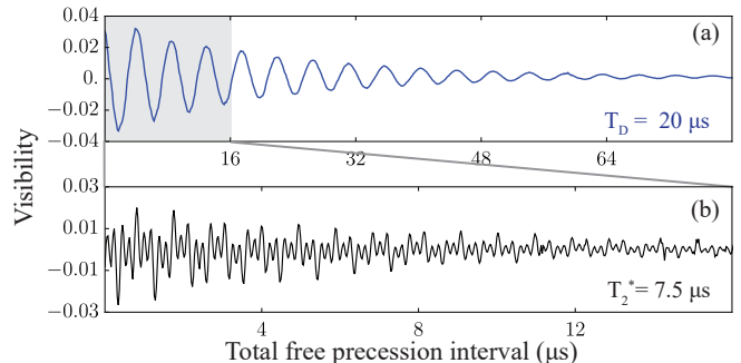
FIG. 7. Comparison of free induction decays for different measurement protocols. (a) Visibility ( \nu ) as a function of evolution time for the strain-CPMG sequence with common MW detuning \delta_{\text{cm}} = 0.35 MHz, yielding a determination of T_D . (b) SQ measurement, addressing the |0\rangle \leftrightarrow |+1\rangle transition with 3 MHz detuning, providing a determination of T_2^* . The visibility oscillates as a superposition of three frequencies, each of which are detunings from hyperfine splittings. The SQ measurement result is shown for the first 16 \mu\text{s} , addressing the same period as that shown in the gray shaded region in (a) for the strain-CPMG measurement result.
